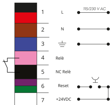
Distributor Control CN1
