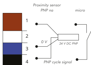
External Pulse Control CN2
