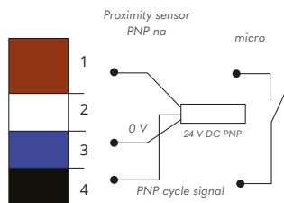
Distributor Control CN1
